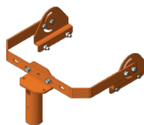
Support poteau 1 SBT2-F-0/G SBT-PLB80-0/G
